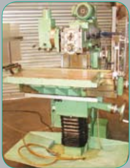
BEAVER VANTAGE model X8140 Universal Toolroom Miller, (Decklele type machine) Table 800 x 400mm. £4950
